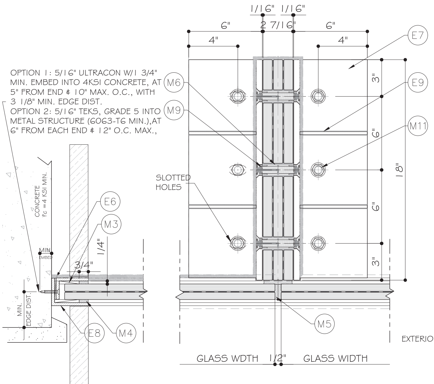
8 D4 DETAIL
