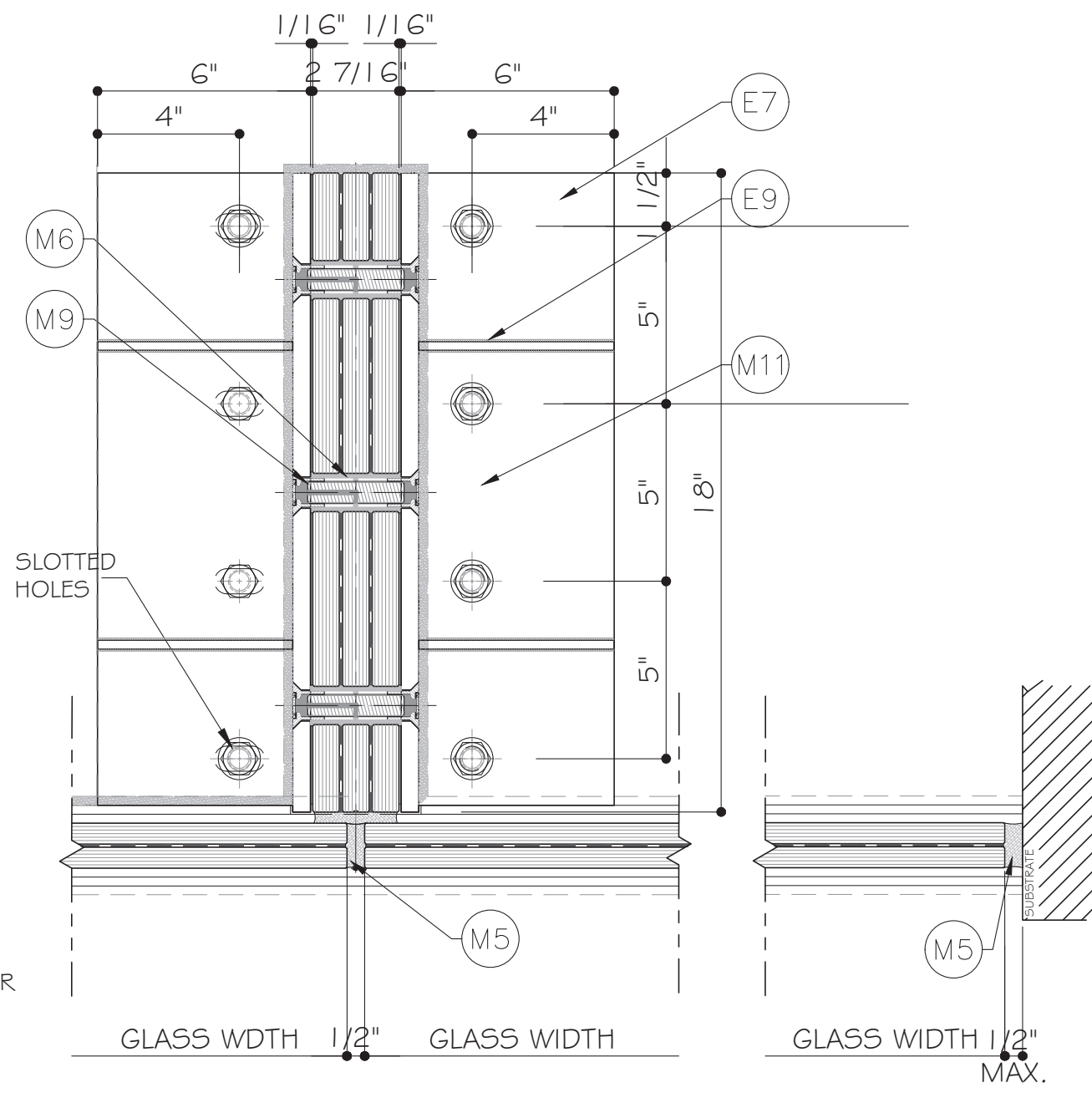
9 D4 DETAIL
